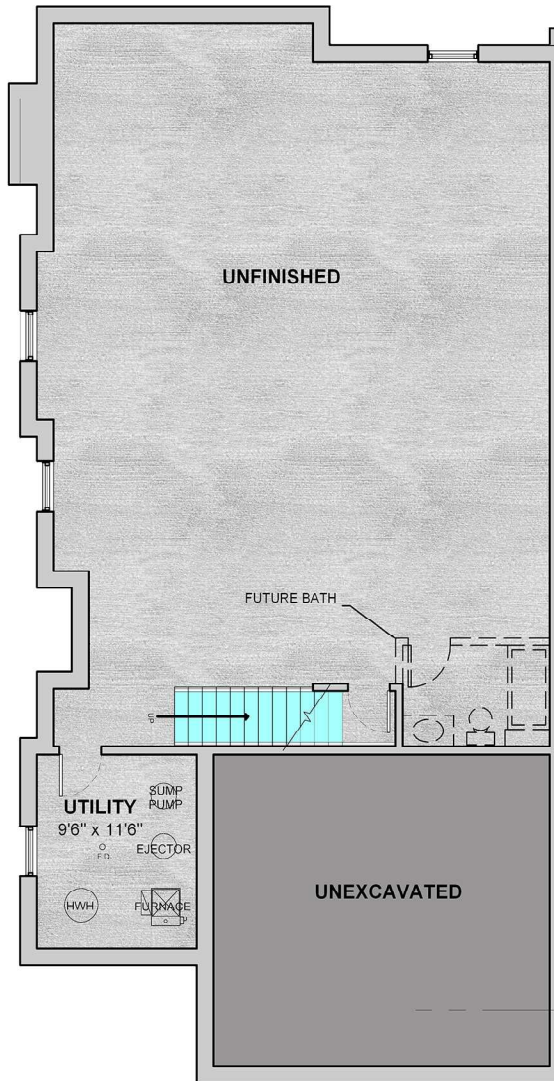
Lower Level
